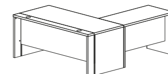
DESK COMPOSITION 1 PJTI0815GR Desk + Return desk inch W 81" D 71" H 30" cm L 206 P 180 H 76 Crts 4 kg 130 m 3 0,43
