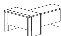
DESK COMPOSITION 3 PJTI0817GR Desk + Return desk inch W 71" D 47" H 30" cm L 181 P 120 H 76 Crts 4 kg 95 m 3 0,31
