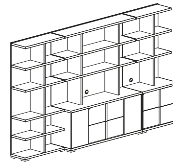
LIBRARY COMPOSITION 3 PJTI0802GR inch W 146" D 20" H 84" cm L 369,4 P 52 H 212,2 Crts 10 kg 468 m 3 2,20
