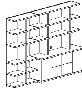
LIBRARY COMPOSITION 5 PJTI0804GR inch W 110" D 20" H 84" cm L 279,6 P 52 H 212,2 Crts 7 kg 335 m 3 1,55
