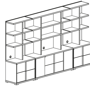
LIBRARY COMPOSITION 2 PJTI0801GR inch W 142" D 20" H 84" cm L 359,2 P 52 H 212,2 Crts 10 kg 510 m 3 2,47
