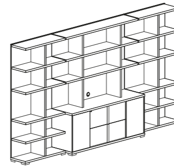
LIBRARY COMPOSITION 1 PJTI0800GR inch W 150" D 20" H 84" cm L 379,6 P 52 H 212,2 Crts 10 kg 428 m 3 1,93
