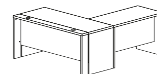
DESK COMPOSITION 2 PJTI0816GR Desk + Return desk inch W 77" D 66" H 30" cm L 196,2 P 167 H 76 Crts 4 kg 118 m 3 0,39
