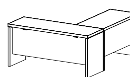
DESK COMPOSITION 2 PJS0912 Desk + Return desk inch W 66" D 77" H 30" cm L 167 P 196,2 H 75,9 Crts 2 kg 119 m 3 0,37
