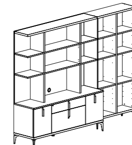
LIBRARY COMPOSITION 6 PJMM0805 inch W 110" D 20" H 84" cm L 279,6 P 52 H 212,2 Crts 7 kg 278 m 3 1,37
