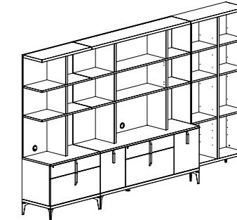
LIBRARY COMPOSITION 4 PJMM0803 inch W 146" D 20" H 84" cm L 370,2 P 52 H 212,2 Crts 10 kg 385 m 3 1,96
