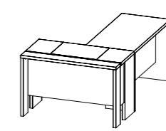
DESK COMPOSITION 3 PJMM0817 Desk + Return desk inch W 71" D 47" H 30" cm L 181 P 120 H 76 Crts 4 kg 91 m 3 0,33
